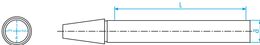
▲ Test bars with 7/24 taper No. 2102
