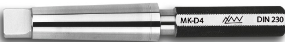
▲ Morse taper plug gauge with tang No. 1310
