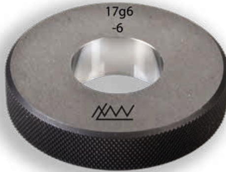
▲ Go ring gauge No. 1140
